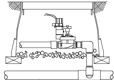
Plastic Electric Remote Control PEBIVM or PESBIVM Valve (with PRS-D)
