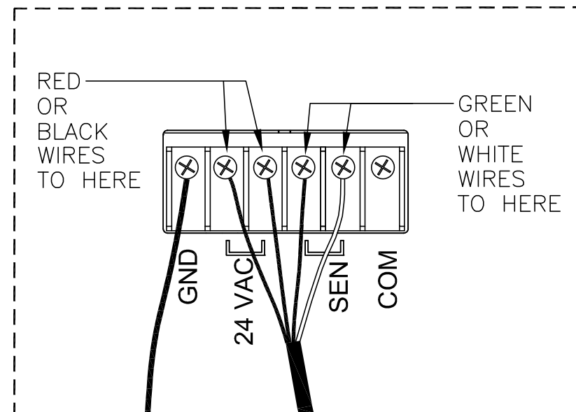
WIRING DETAIL
