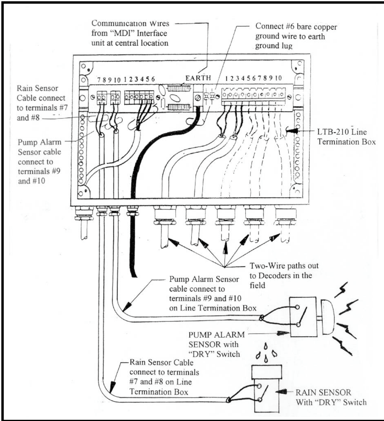
SENSOR CONNECTIONS TO LINE TERMINATION BOX FIGURE: 6.4
