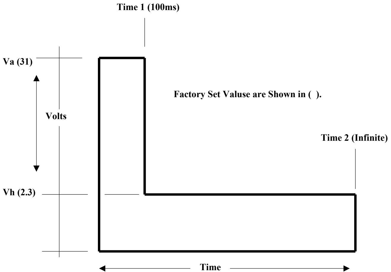
Activating Voltage for Solenoid or Relay FIGURE: 6.1
