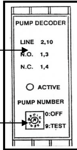
PUMP DECODER FACE FIGURE: 6.3
