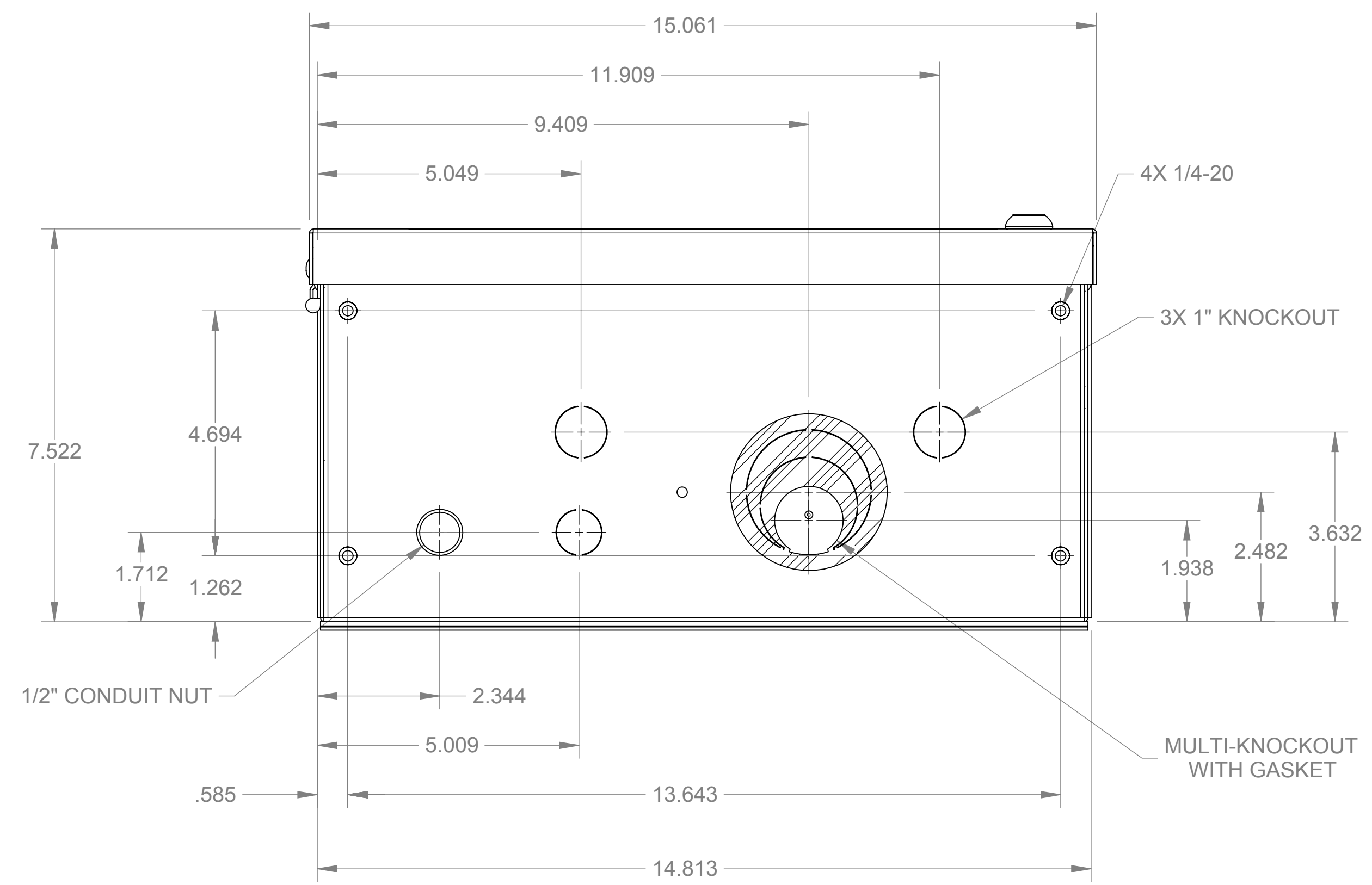
LXMM BOTTOM VIEW
